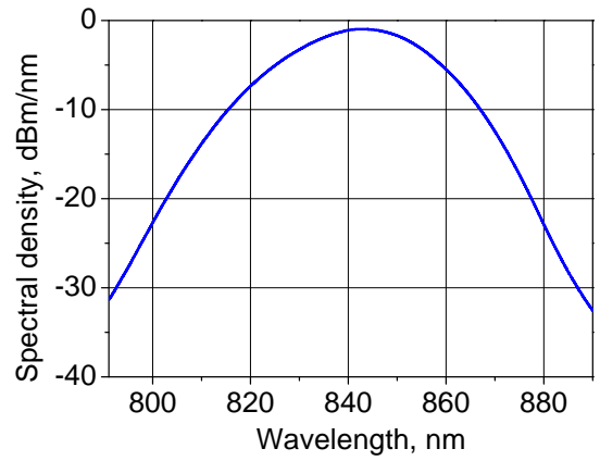
Spectral density at 25 mW power level
