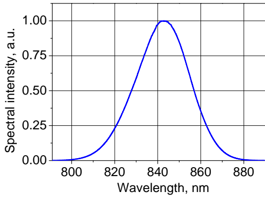
Spectrum at 25 mW power level
