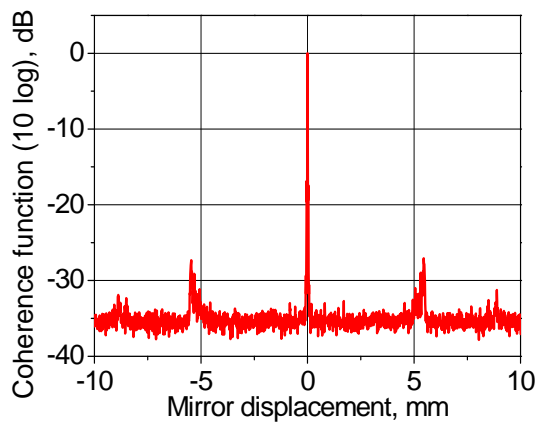
Coherence function at 25 mW power level (extended displacement)
