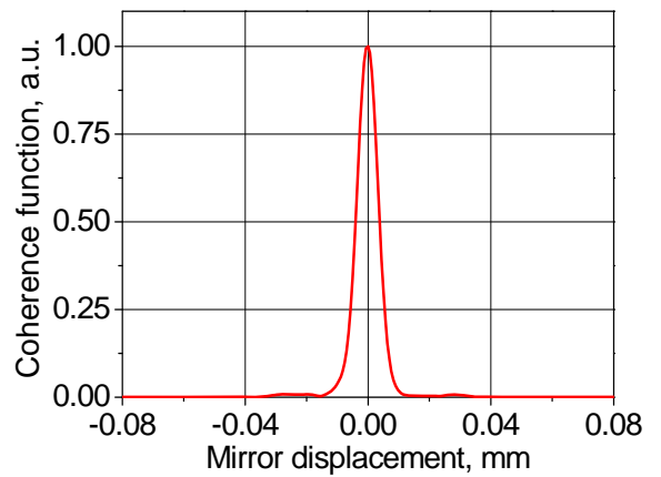
Coherence function at 25 mW power level (short displacement)
